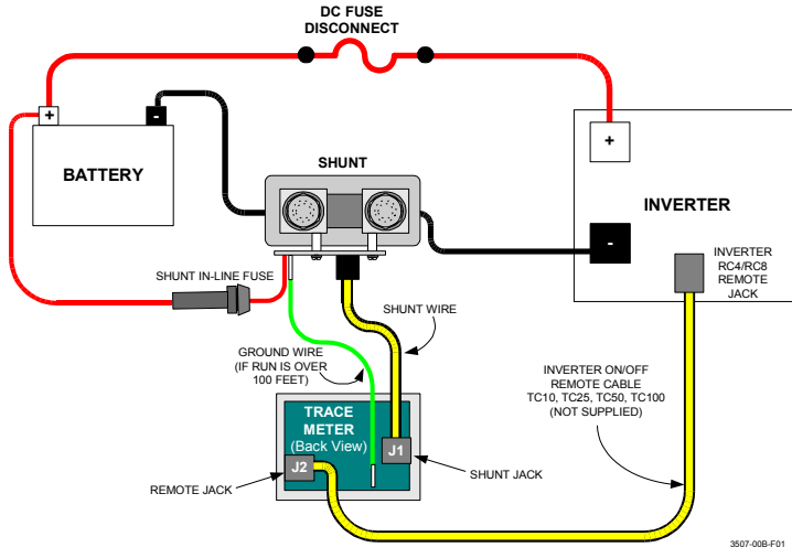
Figure 2-10 Circuit Diagram
