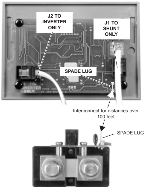
Figure 2-6 Extended Length Ground Wire
