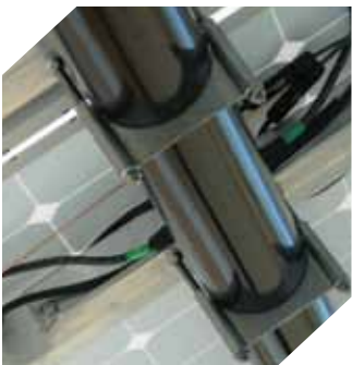
Rail-To-Pipe brackets
