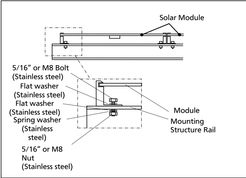
Figure 1-2. Installation
