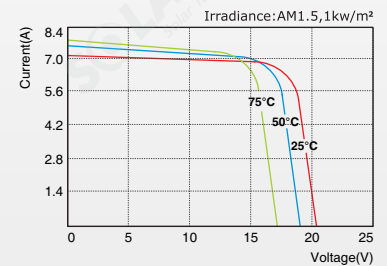
SLP110-12U I-V Curves
